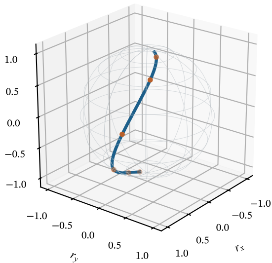
The same path in the Bloch sphere
