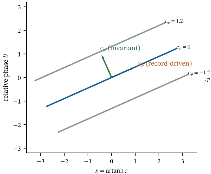
QND trajectories are translations
